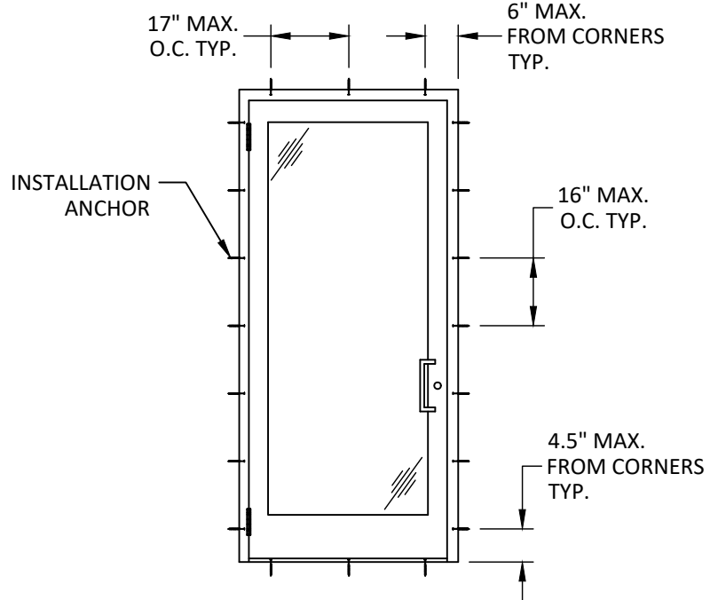
ANCHOR LAYOUT
