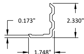
17 THRESHOLD CLIP
