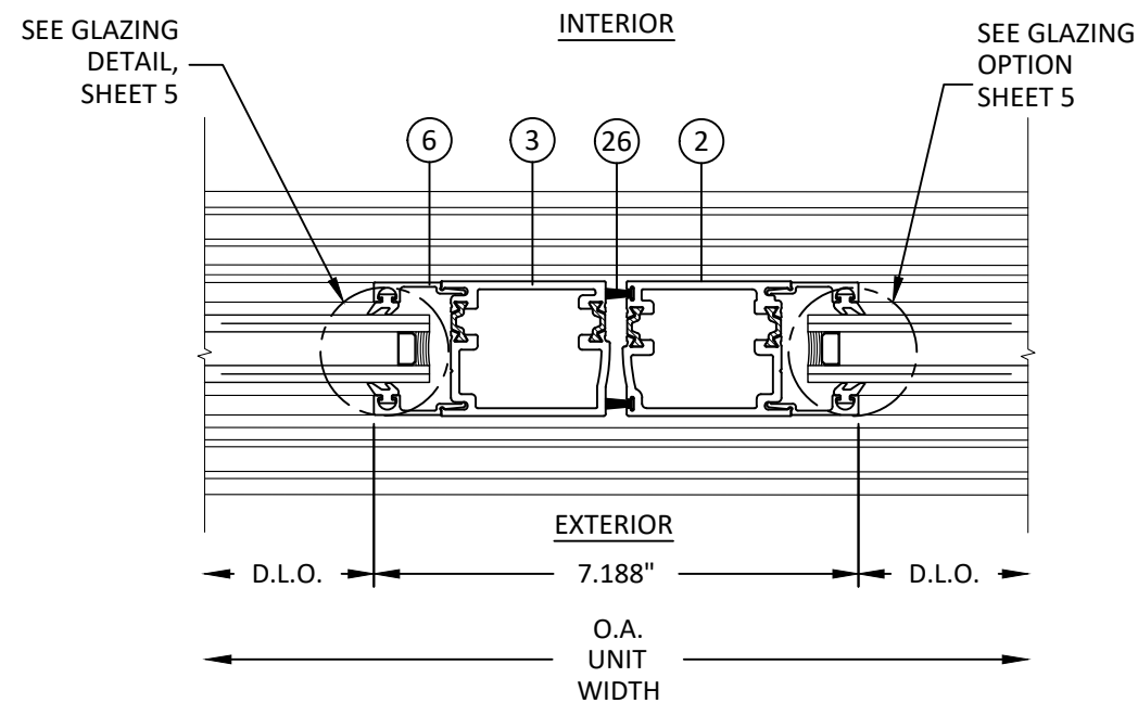
J 6 HORIZONTAL SECTION STANDARD MEETING STILE
