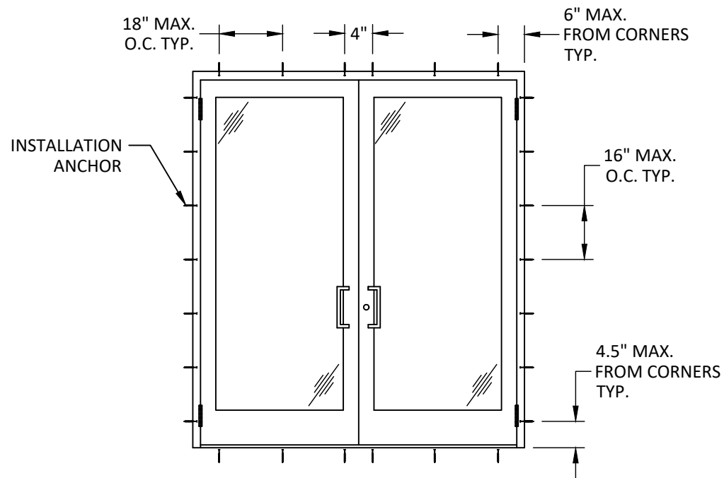
ANCHOR LAYOUT
