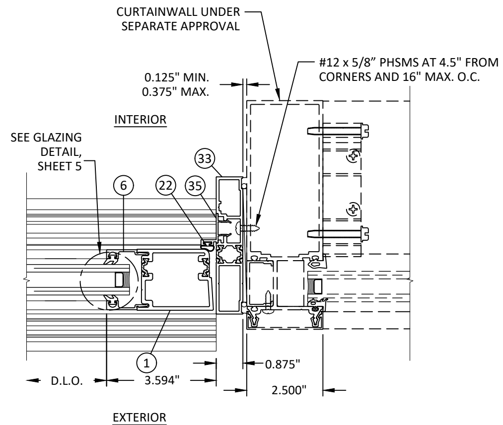
K 7 HORIZONTAL SECTION STANDARD LOCK OR HINGE JAMB THERMAL JAMB SUBFRAME (FLAT) TO CURTAINWALL
