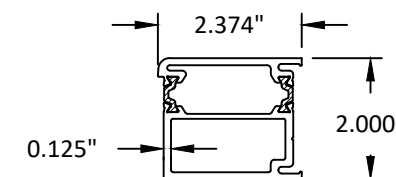
30 CONTINUOUS HINGE STILE
