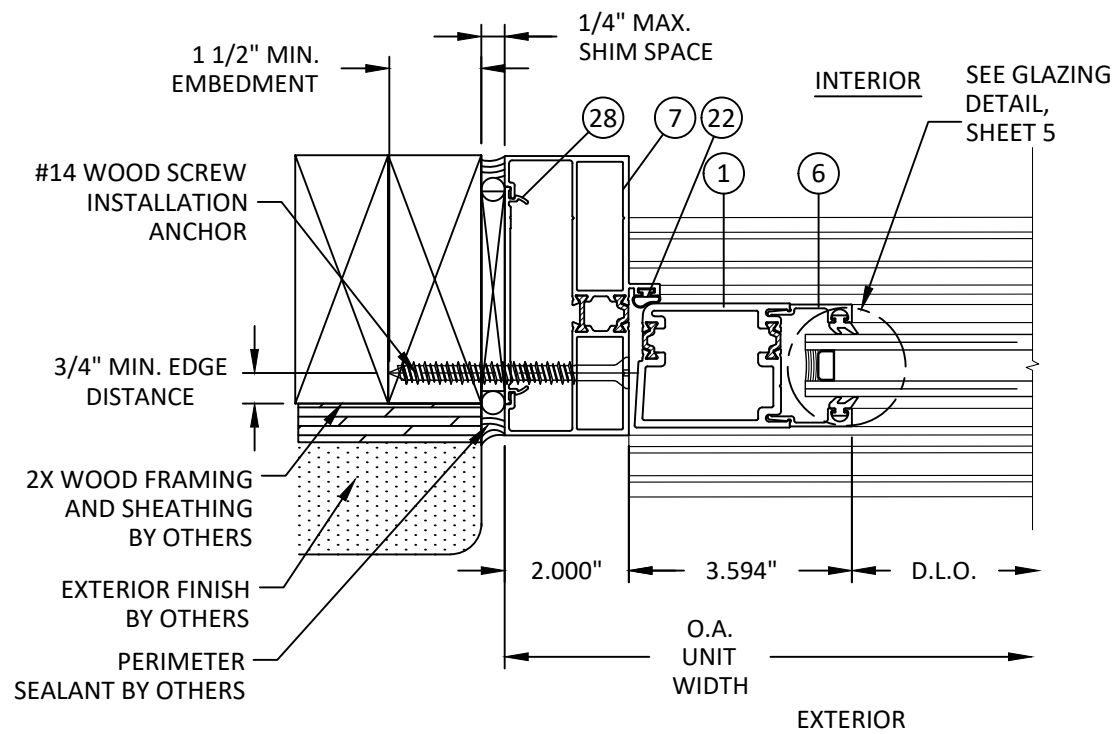
G 6 HORIZONTAL SECTION STANDARD HINGE OR LOCK JAMB WOOD FRAMING
