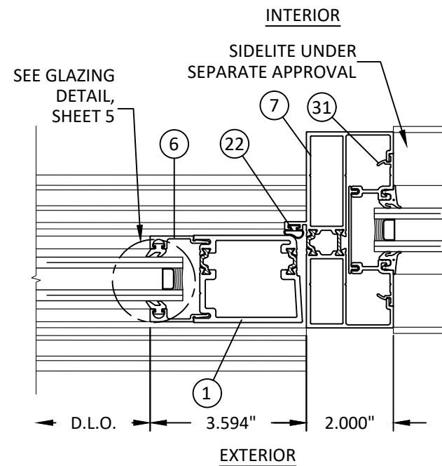
H 6 HORIZONTAL SECTION STANDARD LOCK OR HINGE JAMB WITH SIDELITE (YES 45 TU/XT SHOWN, OTHER OPTIONS AVAILABLE. SEE SEPARATE FRAMING APPROVALS)
